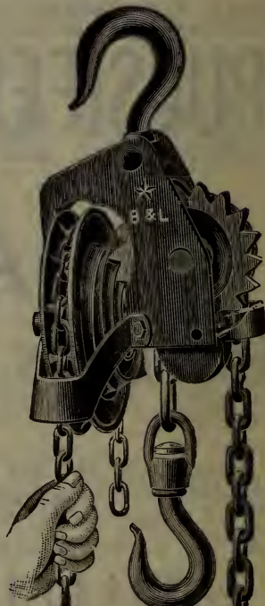
Improved Differential Hoist with Self- Lubricating Bearings.
